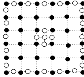
Fig 2. Newly-added nodes by adaptive refinement strategy.
