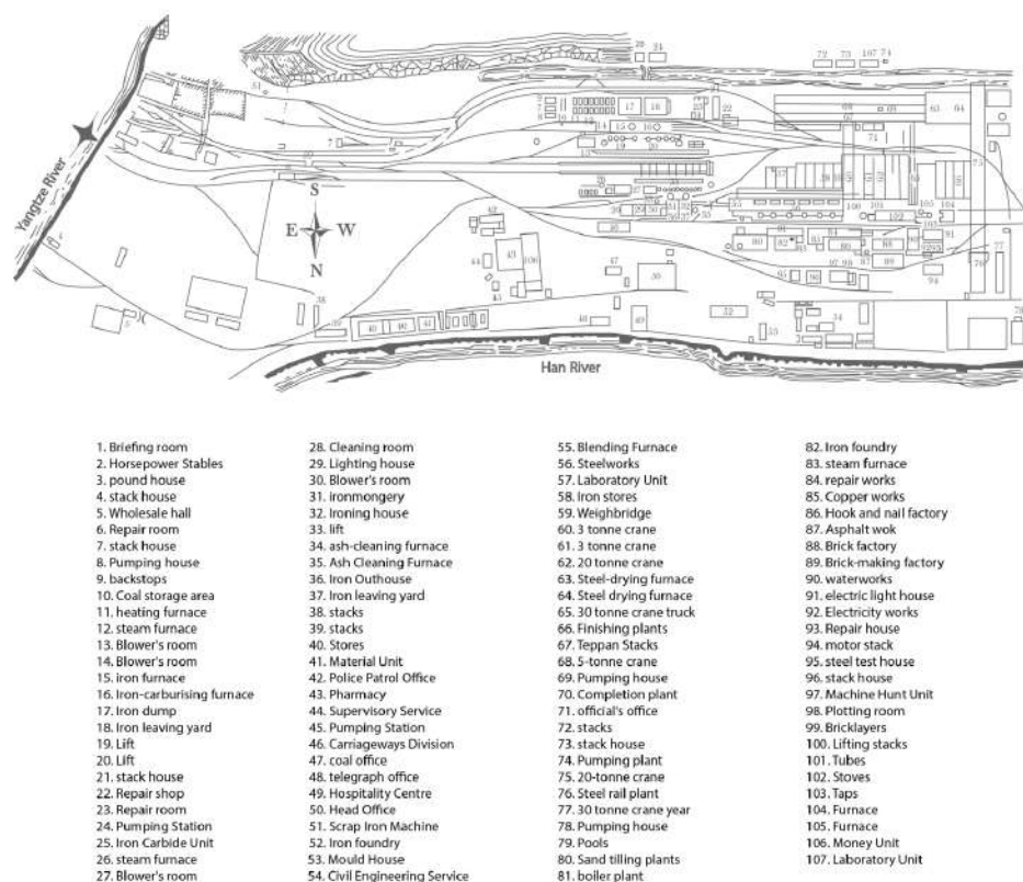
Site Plan of the Expanded Hanyang Ironworks
