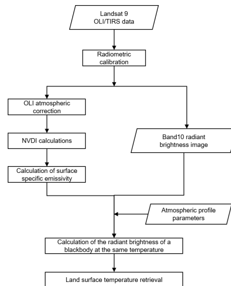
Fig. 4. Workflow of satellite image processing for land surface temperature
