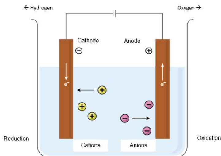
Figure 1: Basic design for water electrolysis (Vögtl, Dr. A., 2024), with own modifications
