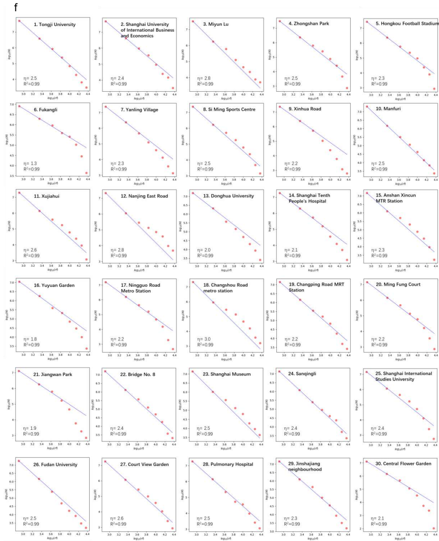
Fig.1| The scaling laws of bike-sharing visitations. a , The power-law distribution between travel distance r and bike visitations. b , The power-law distribution between frequency f and bike visitations. c , For a fixed f , the bike visitations N_i(r, f) , decreases with increasing r with a fixed exponent. d , The empirical distribution of power-law exponents \eta . e , The fitting R^2 of the distance–frequency distribution. f , The Distance-frequency laws of top 30 grids in Shanghai.
